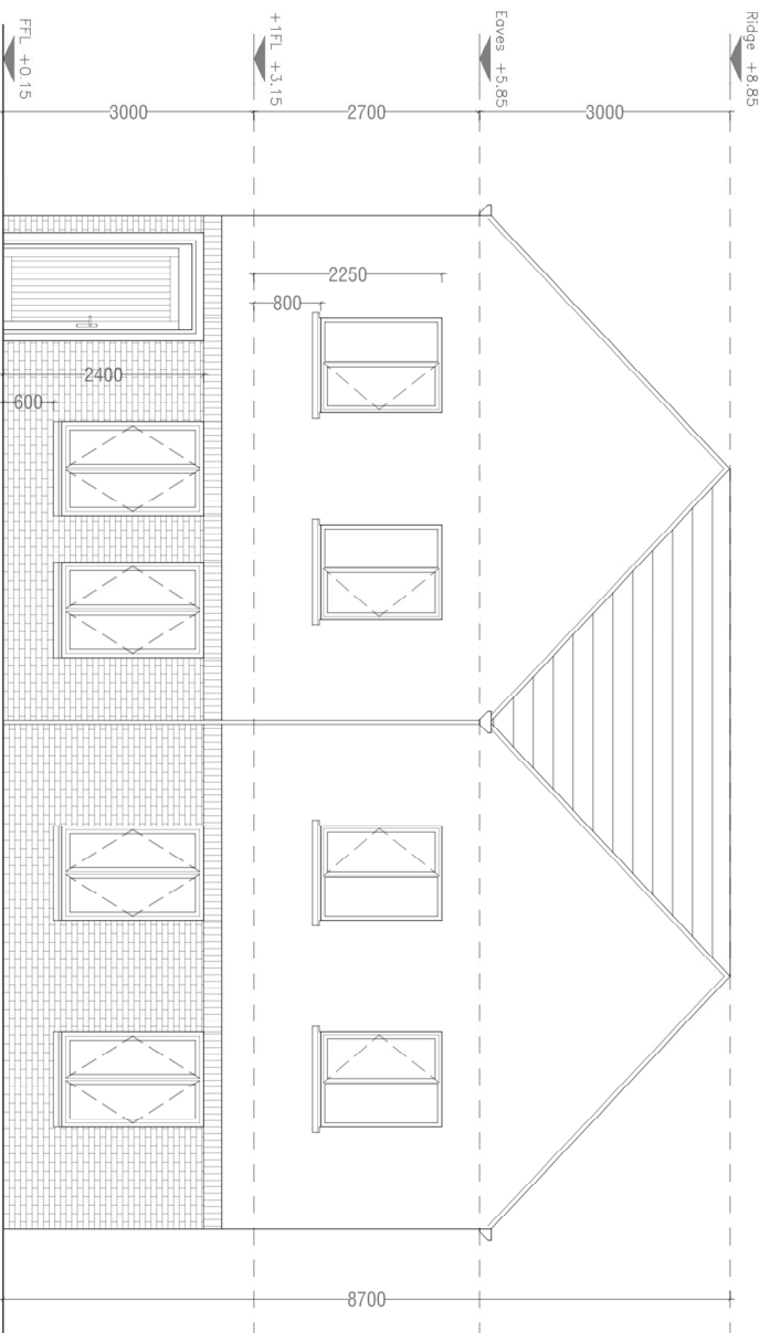
House Type N1 Semi-Detached Front Elevation
