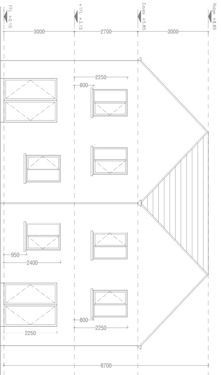
House Type L1 Semi-Detached Rear Elevation
