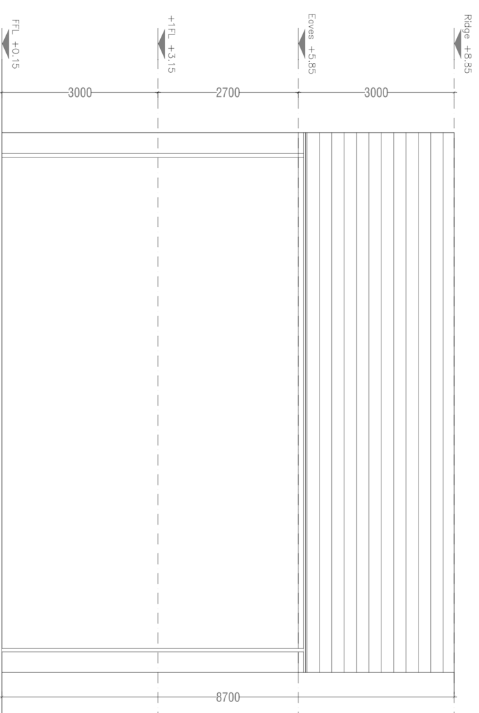
House Type N1 Semi-Detached Side Elevation
